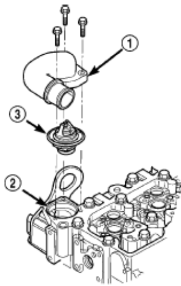
Fig. 22 Thermostat-5.9L Diesel-Typical
