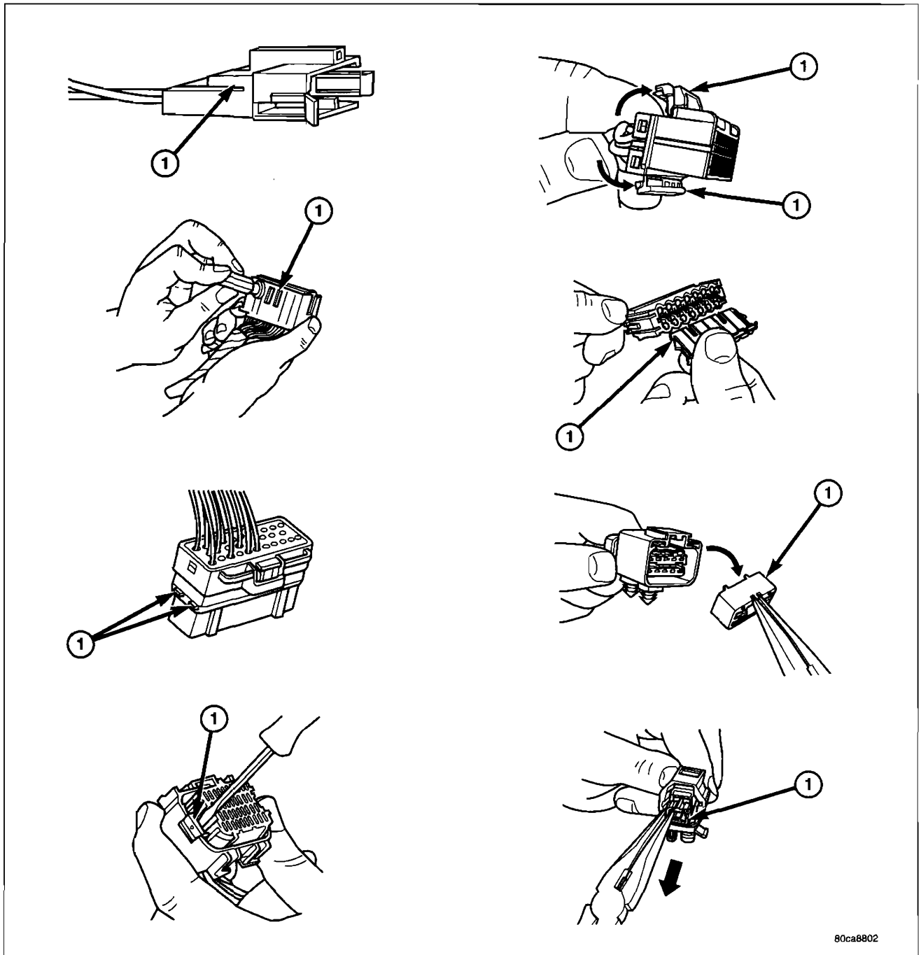
5. Release the Secondary Terminal Lock, if required (1).
